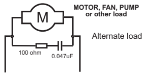
GENERAL WIRING WITH 2 ON-BOARD HIGH POWER ISOLATED RELAYS AND LOW VOLTAGE SUPPLY FOR CONTROLLER
