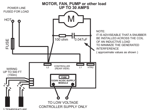
SIMPLE WIRING FOR HIGH POWER AC MOTOR ( or other load ) USING ONLY 1 ON-BOARD HIGH POWER RELAY AND WITH LOW VOLTAGE SUPPLY FOR CONTROLLER
