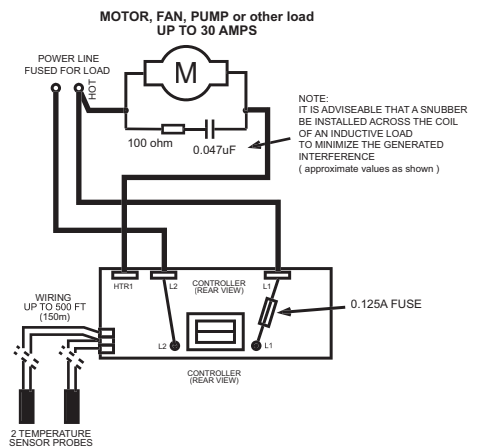
WIRING FOR MOTOR ( FAN or A/C ) or other load ON THE SAME POWER LINE AS CONTROLLER SUPPLY AND USING ONLY 1 ON-BOARD RELAY
